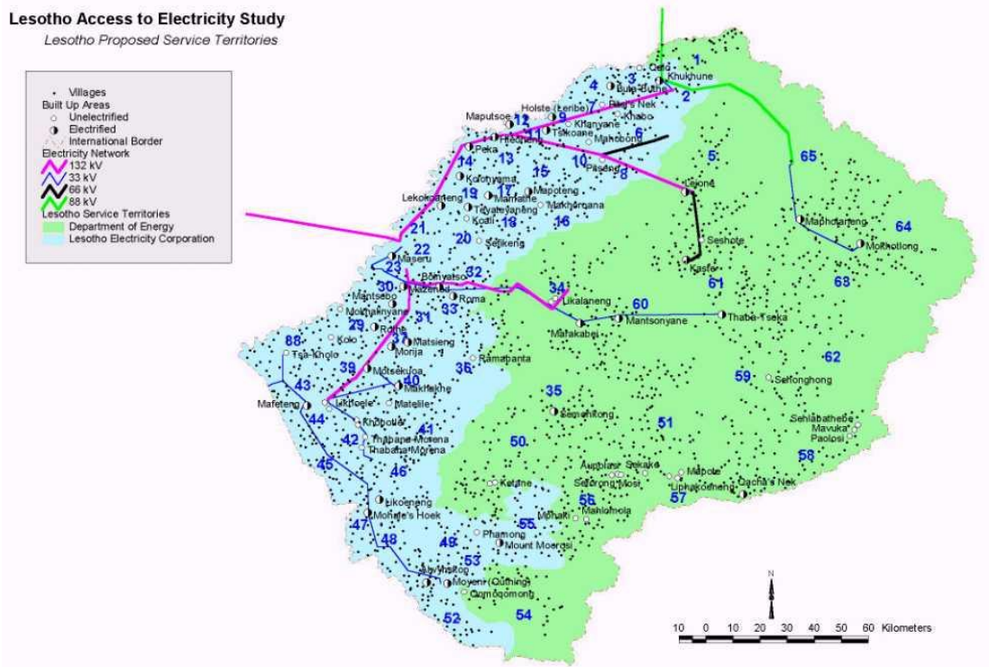
Figure 1 Proposed LEC service territory
